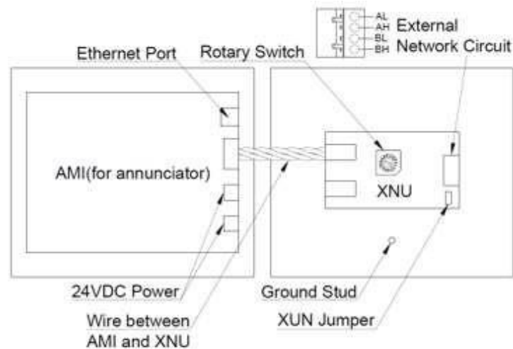
Figure 3. Connection
