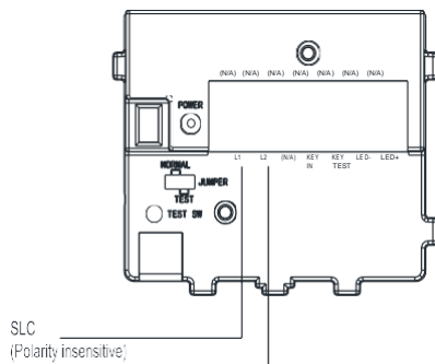
Figure 5 Wiring Diagram
