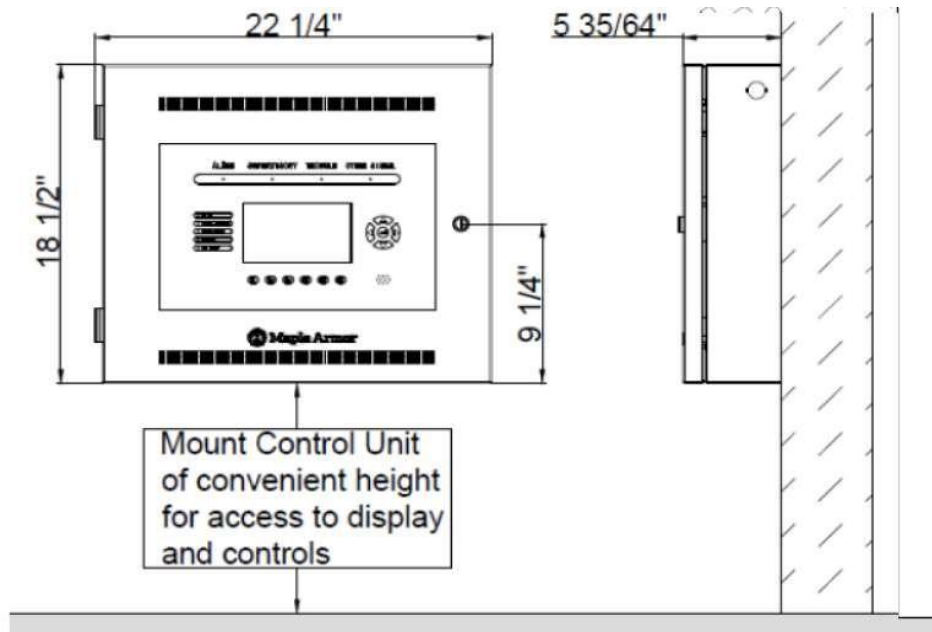
(a) Surface mounting
