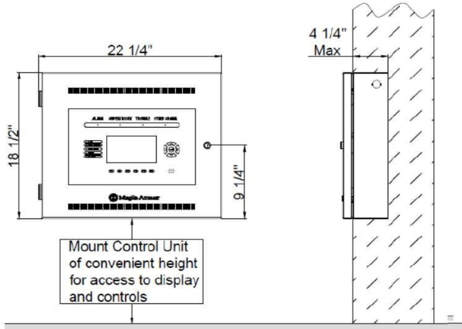
(b) Flush mounting
